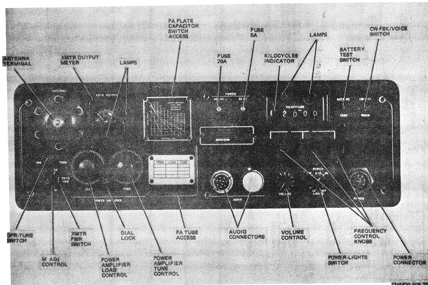
Figure 3-87. Radio Receiver-Transmitter RT-671/PRC-47 (A8), Front Panel View, Location of Access Opening and Panel Components.
