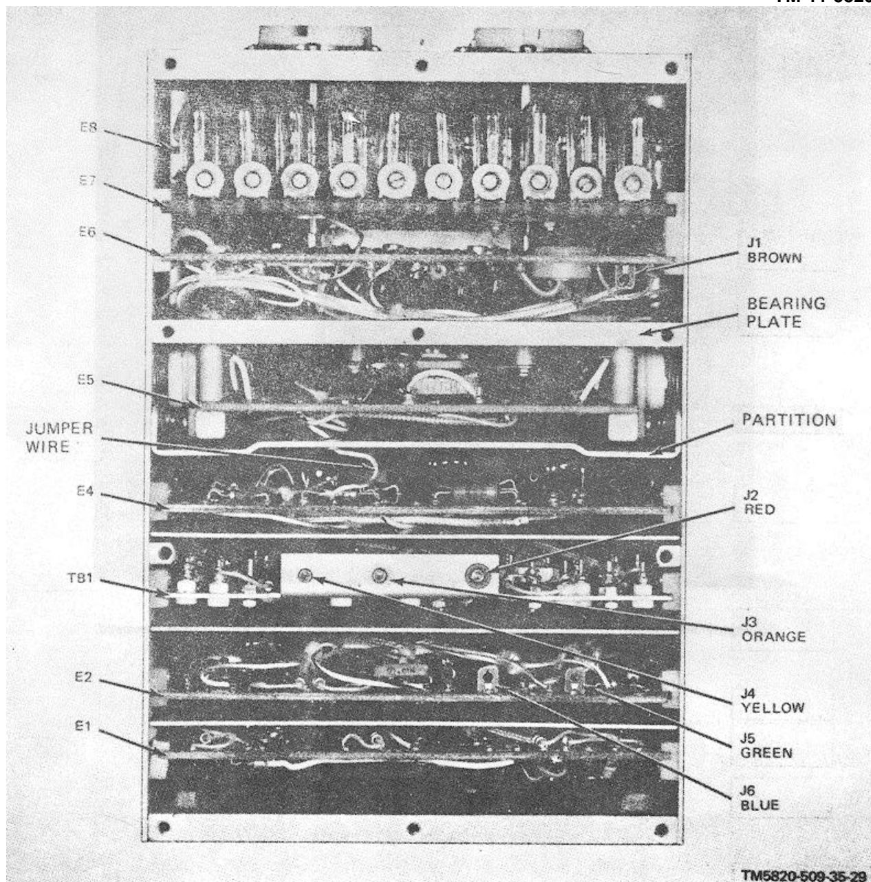
Figure 3-14. Oscillator Control C-4311/PRC-47 (A8A7), Top View, Cover Removed, Location of Subassemblies and Test Points.
